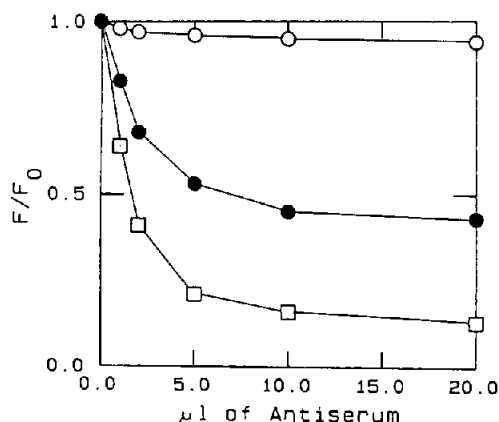
Fig.1. The effect of anti-fluorescein antibodies on the fluorescence emission of fluorescein. Native FITC-ATPase ( \circ ), denatured ATPase ( \bullet ) or free fluorescein ( \square ) (equivalent to 0.06 nmol of fluorescein) were dispersed in 3 ml PBS. Anti-fluorescein antibodies were added sequentially and the fluorescence intensity of the fluorescein was measured.
