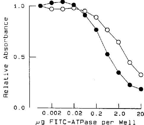
Fig.2. Determination of the accessibility of the FITC-binding site by competitive ELISA. Native ( \circ ) or denatured ( \bullet ) FITC-ATPase was incubated overnight in the presence of anti-fluorescein antiserum (1:50000 dilution). The incubation was transferred to ELISA plates coated with 1 \mu\text{g} of native ATPase and the amount of free anti-fluorescein antibody estimated by ELISA.
